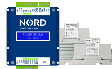
NORD Power Genius 3000 (vč. Solid State Relay)
